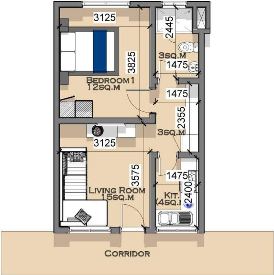
TYPICAL UNIT ONE BEDROOM APARTMENT 42 SQ.M
